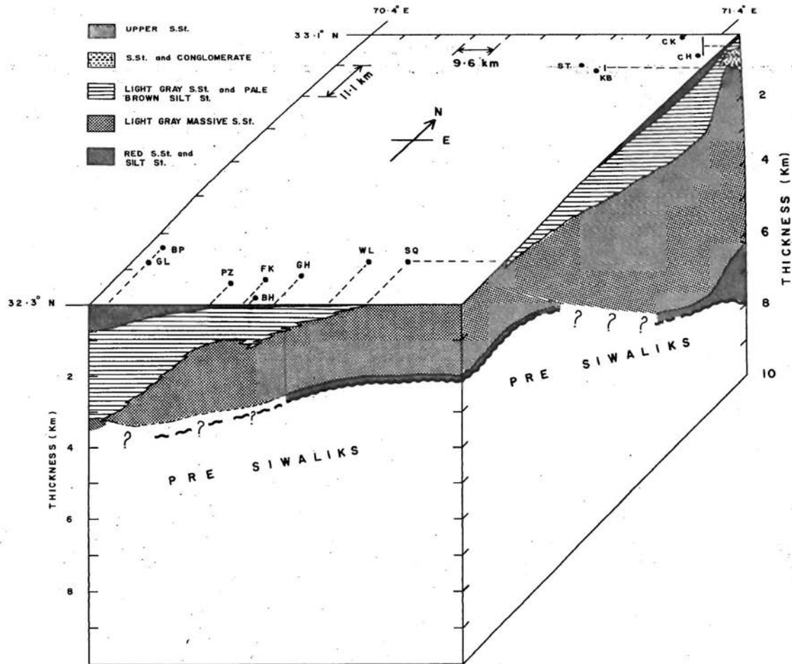
Fig. 2. Block diagram based on the thickness and the dominant lithology of the Siwalik Group exposed in the Trans-Indus Salt Range. Thickness was measured at each corresponding section location. The sections were located at these sites — BH = Bhandara, BP = Bain Pass, CH = Chichali, CK = Chani Khel, FK = Faqir Kili, GH = Gharangai, GL = Garhi Landa, KB = Khora Baroch, PZ = Pezu Pass, SQ = Spin Qammar, ST = Spalmai Tangi and WL = Walewal. The sections measured at KB—ST and CH—CK constitute one stratigraphic sequence each, and therefore data is plotted at an intermediate location.
