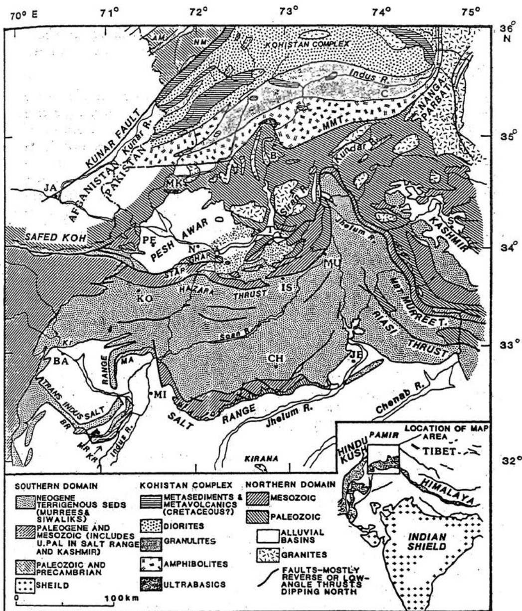
Fig. 1. Geologic sketch-map of northern Pakistan. Adopted from : Gansser (1964), Desio (1964), Calkins, et al. (1975), Tahirkheli and Jan (1979), et al. (1979). Explanations : A = Attock, AM = Asiatic mass, B = Besham, BR = Bhattani Range, CH Chakwal, IS = Islamabad, Ja = Jalabad, JE = Jhelum, KR = Khasor Range, KO = Kohat, KT = Kurram River, MBT = Main Boundary Thrust, MA = Makarwal anticline, MK = Malakand, MR = Marwat Range, MI = Mianwali, MU = Murree, NM = Northern Megashear, N = Nowshera, P = Pattan, PE = Peshawar, S = Srinagar, T = Tarbela.
