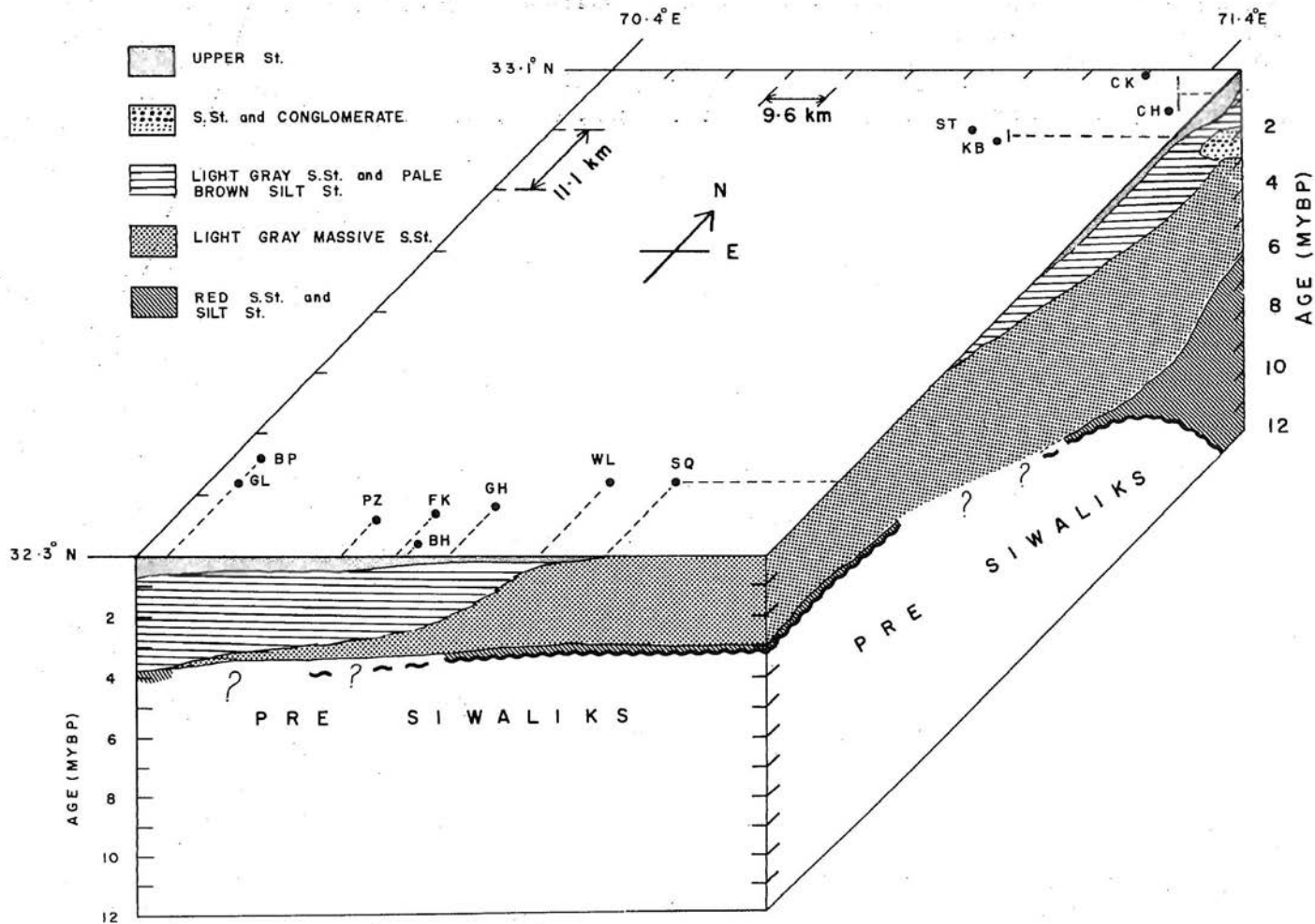
Fig. 3. Block diagram based on the age (after Khan, 1983) plotted against dominant lithology of the Siwalik Group exposed in the Trans-Indus Salt Range. Explanations same as in Fig. 2.
