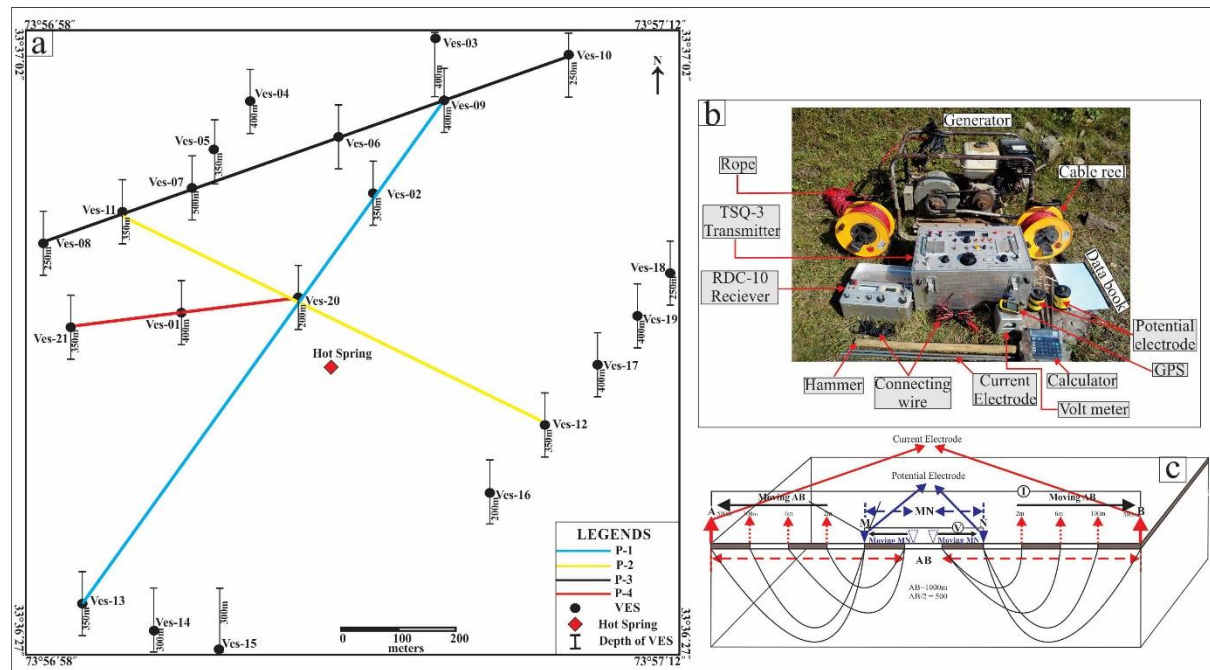
Fig. 2. a) Base Map of the resistivity showing location of VES and 2D profiles, b) Instrumentation utilized for resistivity survey along Tattapani thermal spring, c) Schematic diagram of Schlumberger electrode configuration.
