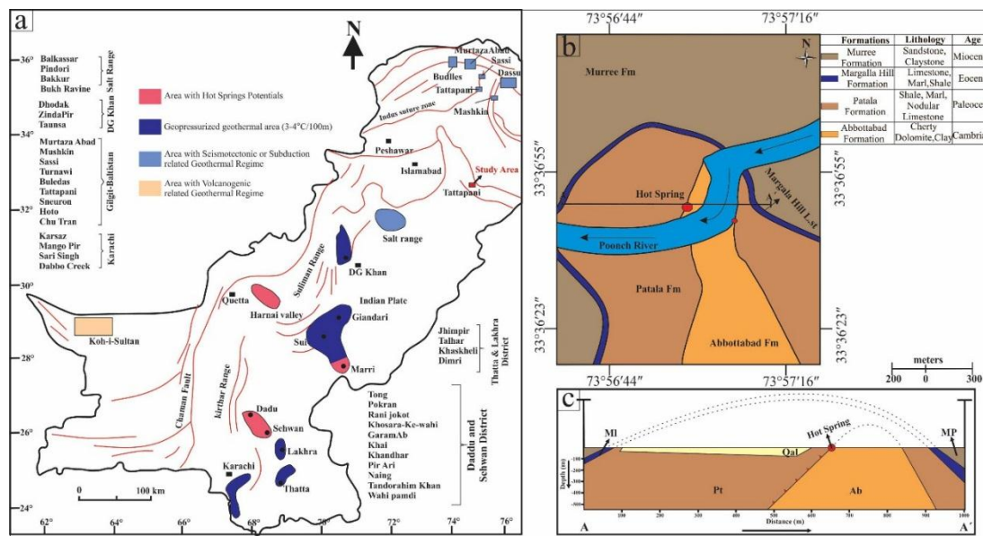
Fig. 1 a) Geothermal Map of Pakistan showing thermal spring Pakistan (Zaigham et al., 2009), b) Geological Map of Tattapani Thermal Spring (Shah et al., 2007), c) Geological Cross-section along Tattapani Thermal Spring (Shah et al., 2007).
