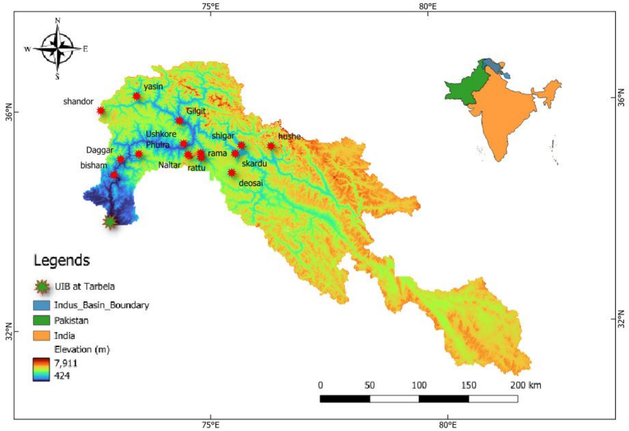
Fig. 1. Spatial distribution of 14 hydrometeorological stations in the upper Indus Basin.
