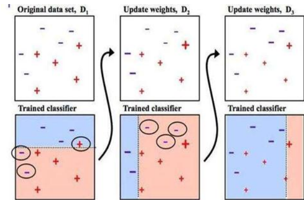
Fig. 6. AdaBoost workflow (Mosavi et al., 2018).
