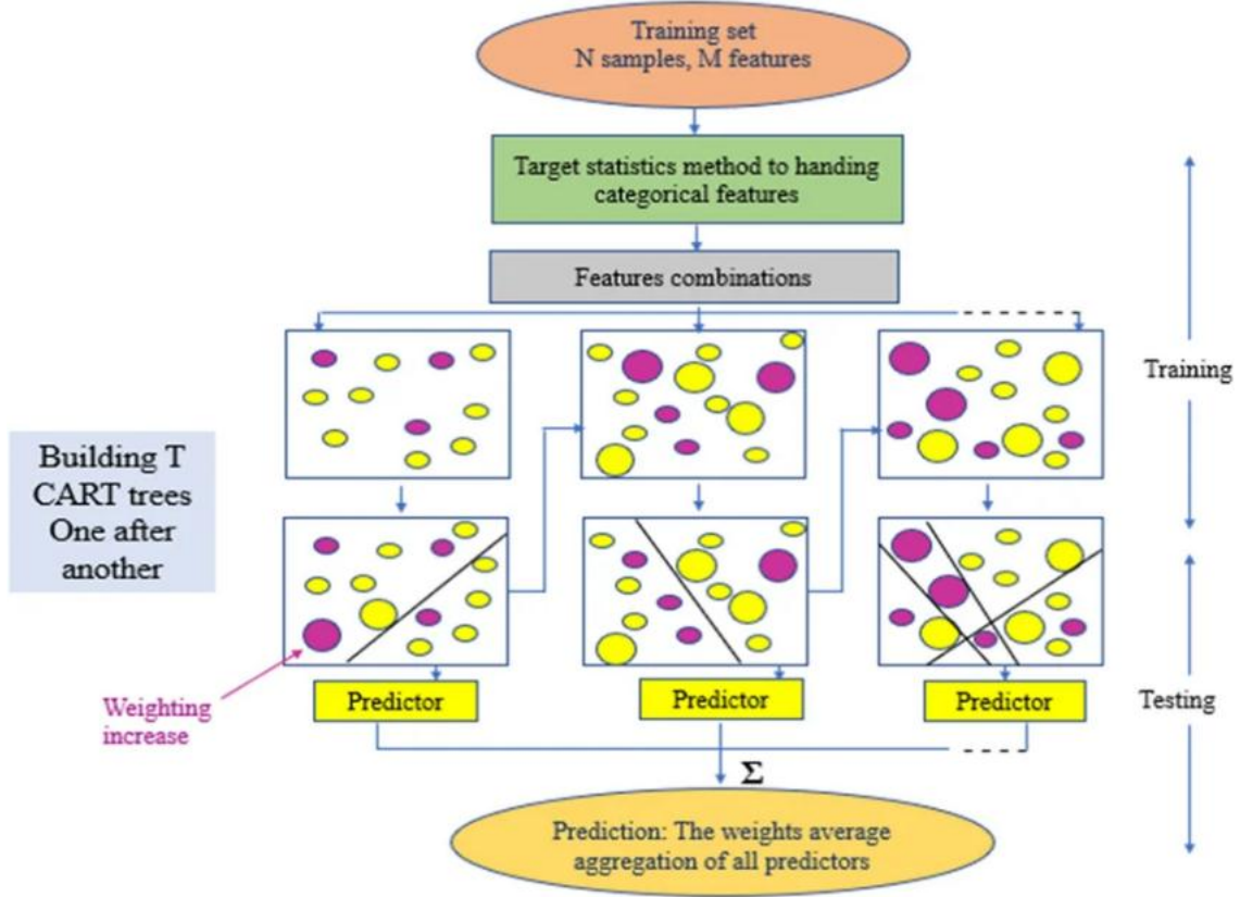
Fig. 3. Catboost workflow (Sireesha et al., 2023).
