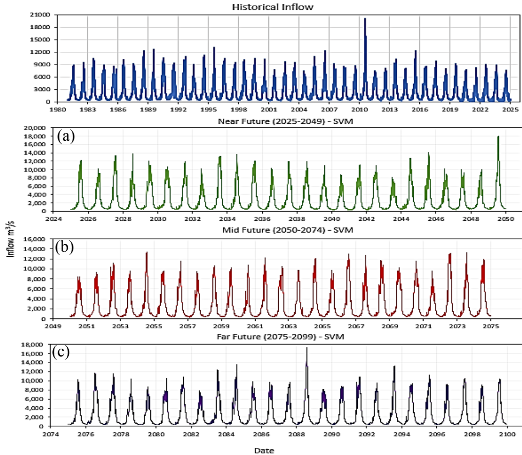
Fig. 20. SVM future inflow prediction under SSP 5-8.5 for (a) Near Future, (b) Mid Future, and (c) Far Future.
