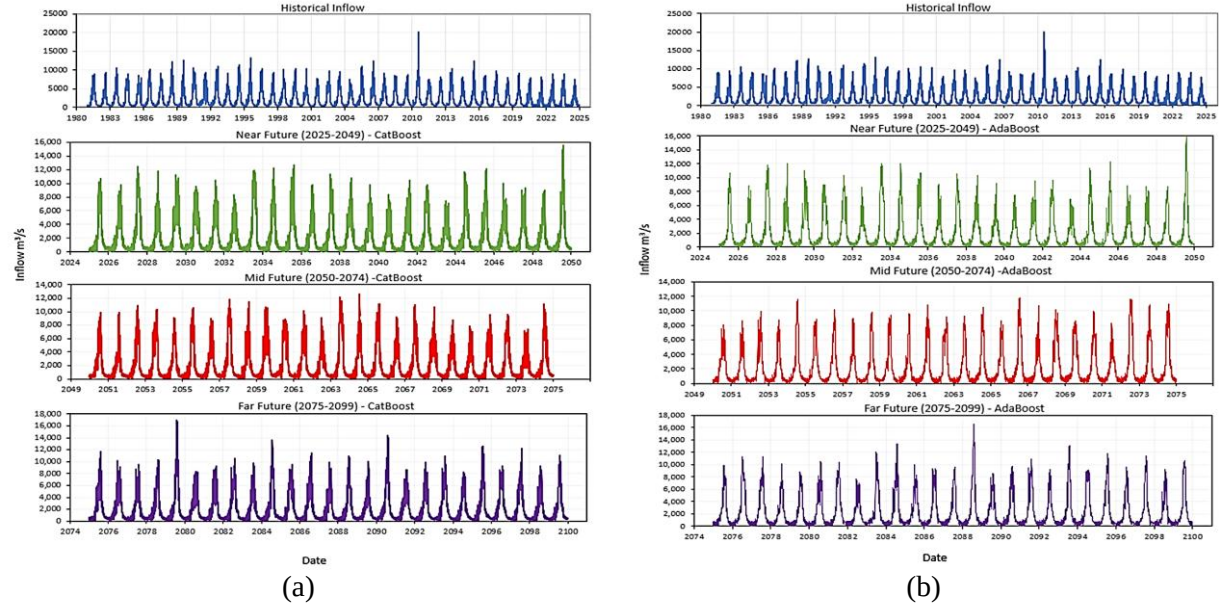
Fig. 12. Near, mid, and far future inflow prediction under SSP 2-4.5 for (a) Catboost and (b) AdaBoost.
