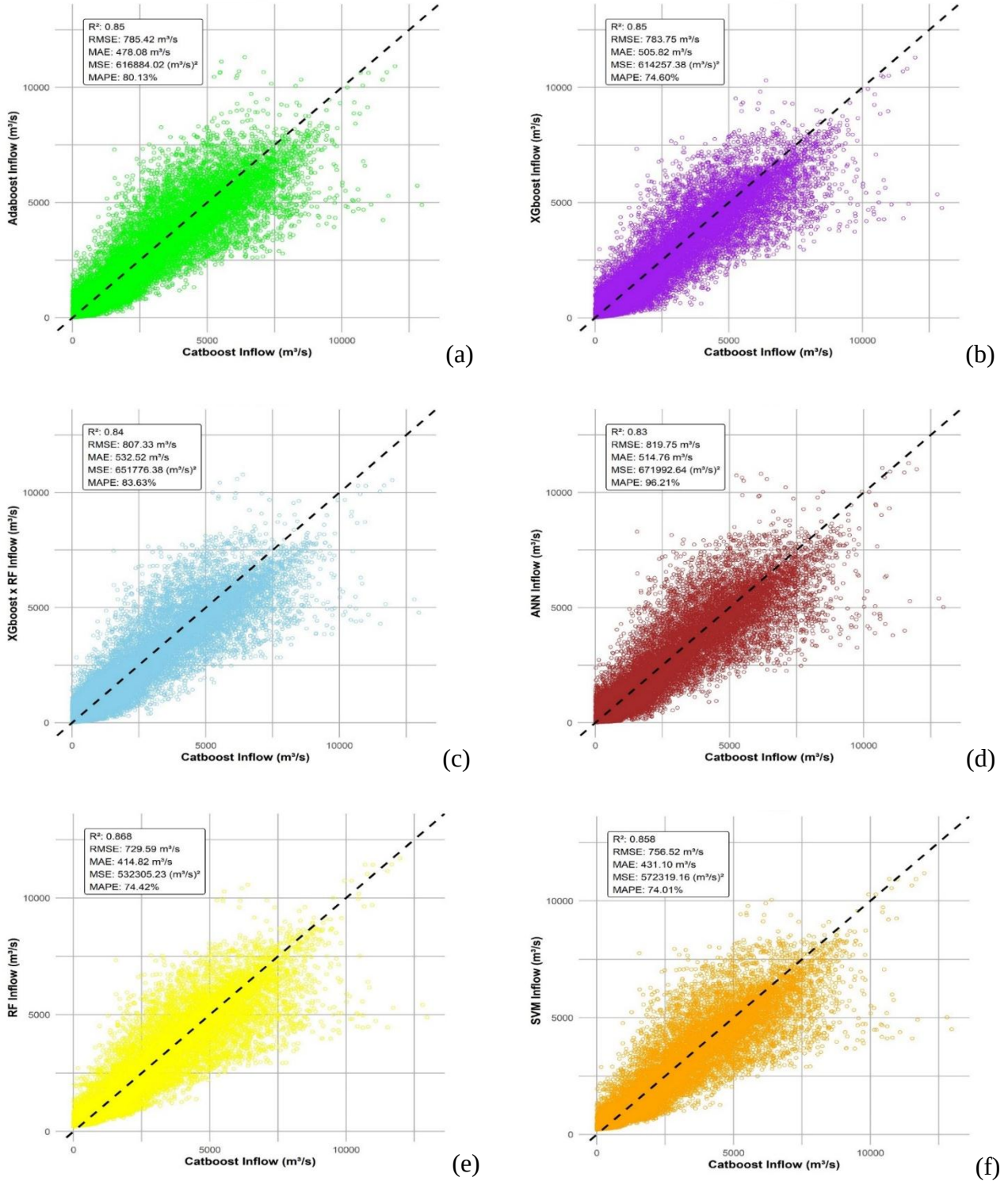
Fig. 16. Scatter plot comparing predicted inflows to Catboost predicted inflows upto year 2100 under SSP 2-4.5. a) AdaBoost, b) XGboost, c) XGboost x RF, d) ANN, e) RF, and f) SVM.
