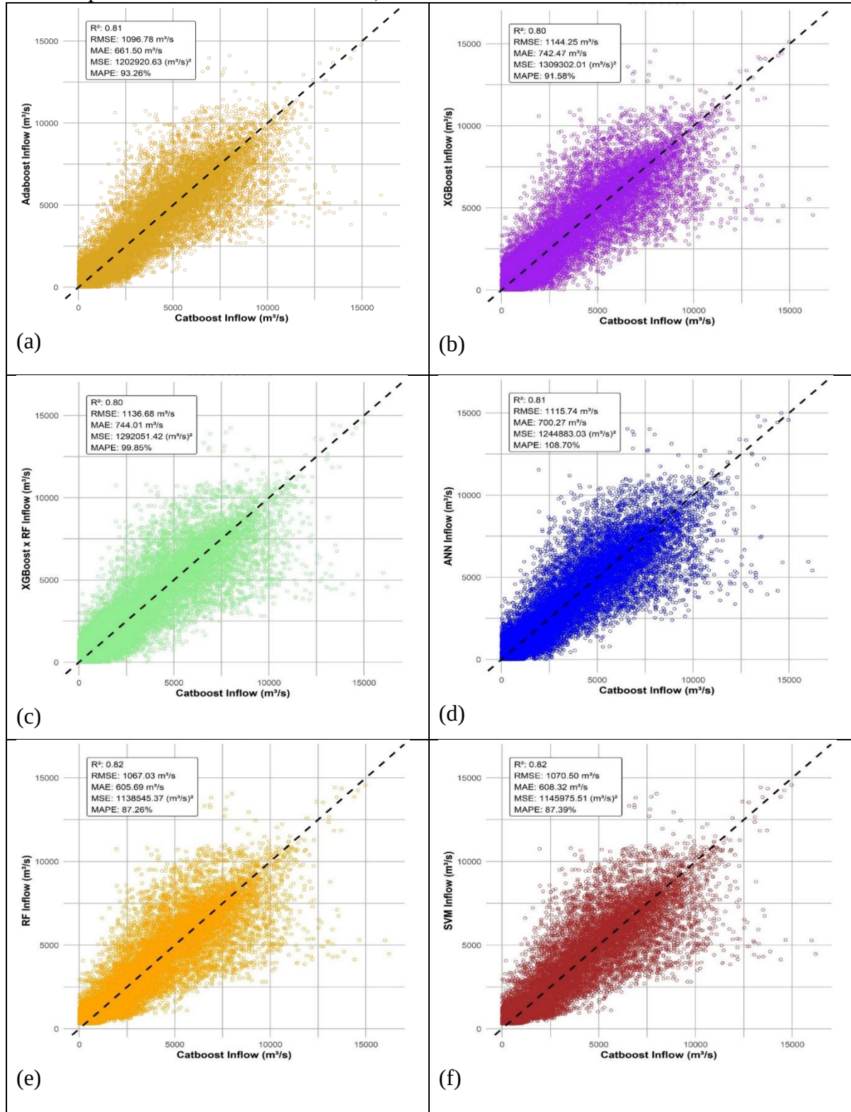
Fig. 21. Scatter plot comparing ML models predicted inflows to Catboost predicted inflows under SSP 5-8.5 upto year 2100. a) AdaBoost, b) XGboost, c) XGboost x RF, d) ANN, e) RF, and f) SVM.
