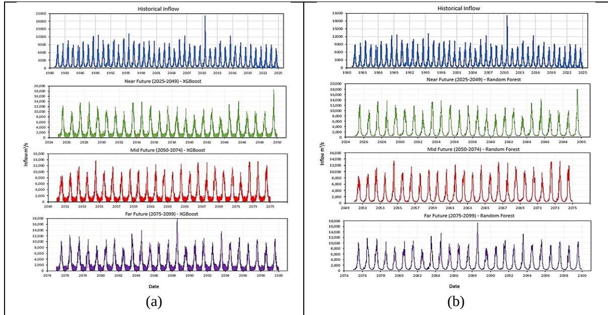
Fig. 18. Future inflow prediction under SSP 5-8.5 under near, mid, and far future for (a) XGBoost (b) Random Forest.
