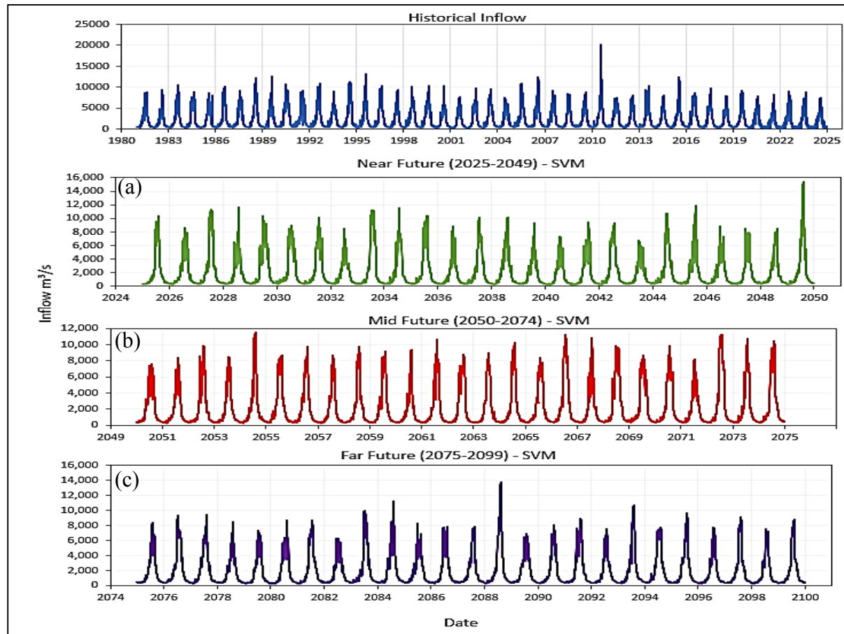
Fig. 15. SVM future inflow prediction under SSP 2-4.5 for a) near, b) mid, and c) far future.
