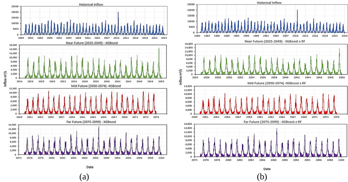
Fig. 13. Near, mid, and far future inflow prediction under SSP 2-4.5 for (a) XGBoost (b) XGBoost and RF Ensemble.
