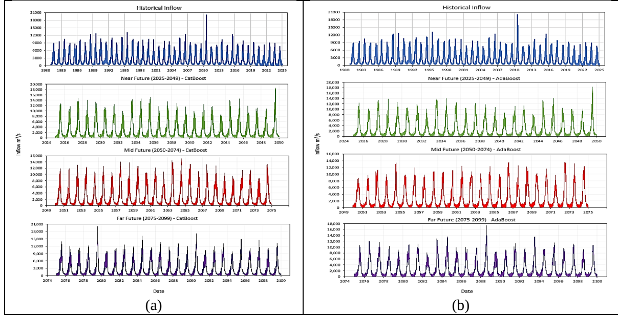
Fig. 17. Future inflow prediction under SSP 5-8.5 under near, mid, and far future for (a) Catboost (b) AdaBoost.
