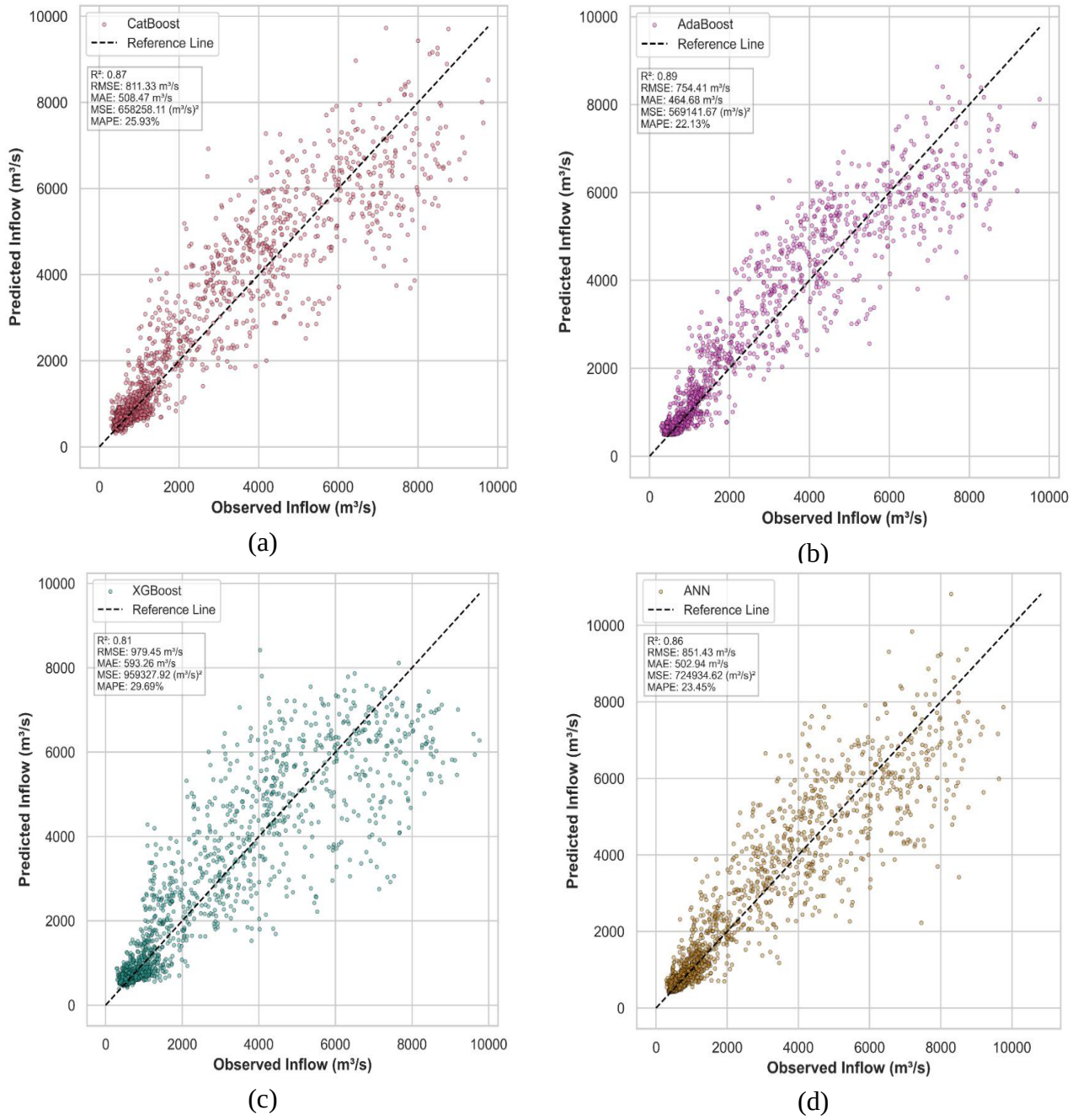
Fig. 11. Scatter plot of observed vs predicted inflows during the testing phase (2016-2020)
