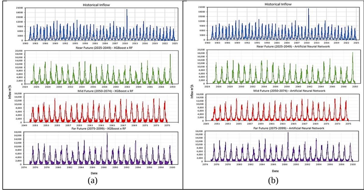
Fig. 19. Future inflow prediction under SSP 5-8.5 under near, mid, and far future for (a) XGBoost RF Ensemble (b) ANN.
