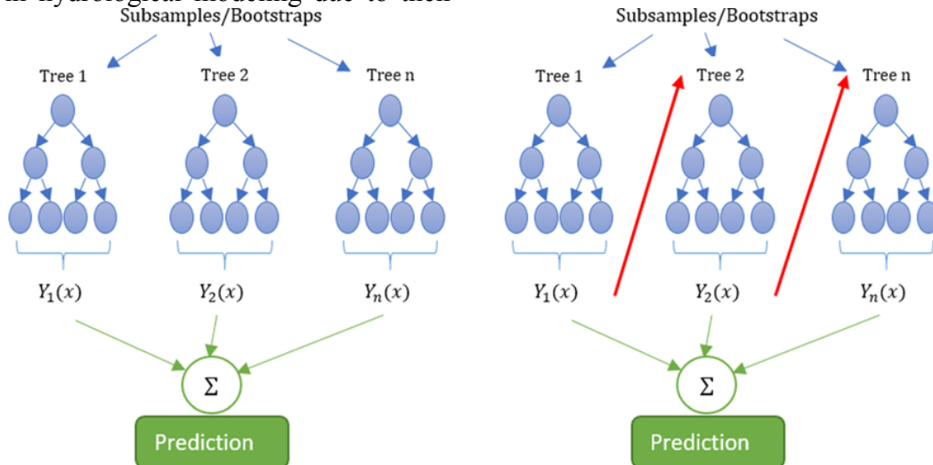
Fig. 8. Random Forest example (left), boosting/XG-boost example (right) (Gupta et al., 2022).
