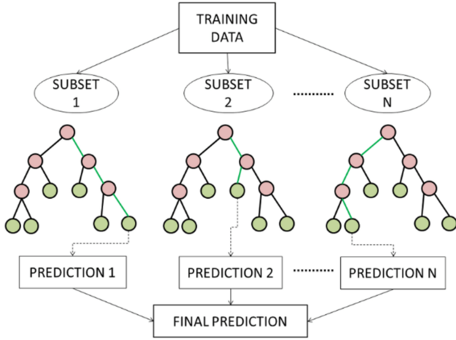
Fig. 4. Random Forest workflow.
