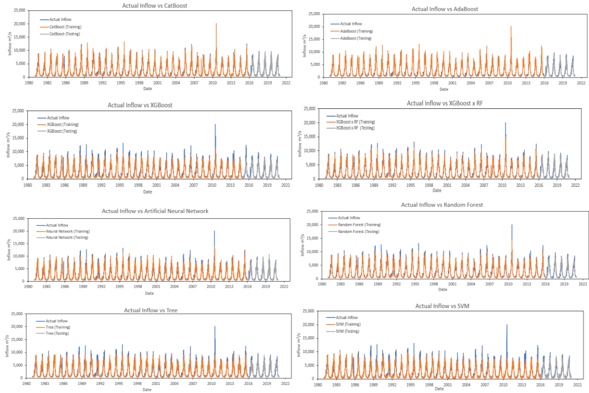
Fig. 9: Training and testing results of all machine learning models vs actual inflow for historical series.
