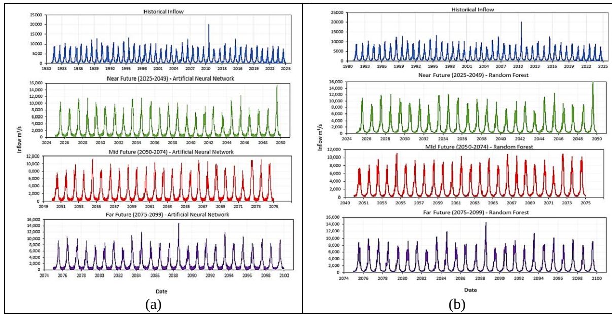
Fig. 14. Near, mid, and far future inflow prediction under SSP 2-4.5 for (a) ANN (b) Random Forest.
